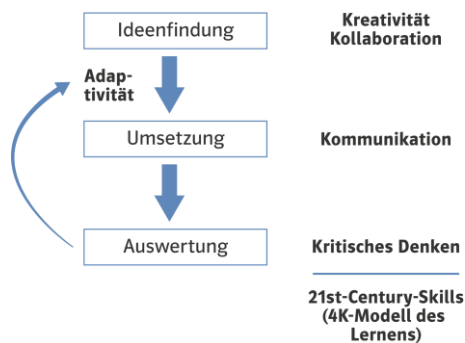
Abb.2: Sprach-KI-Schema
